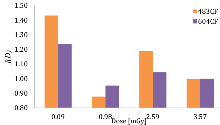
Figure 6. Linearity index of neutron irradiated fibres.
